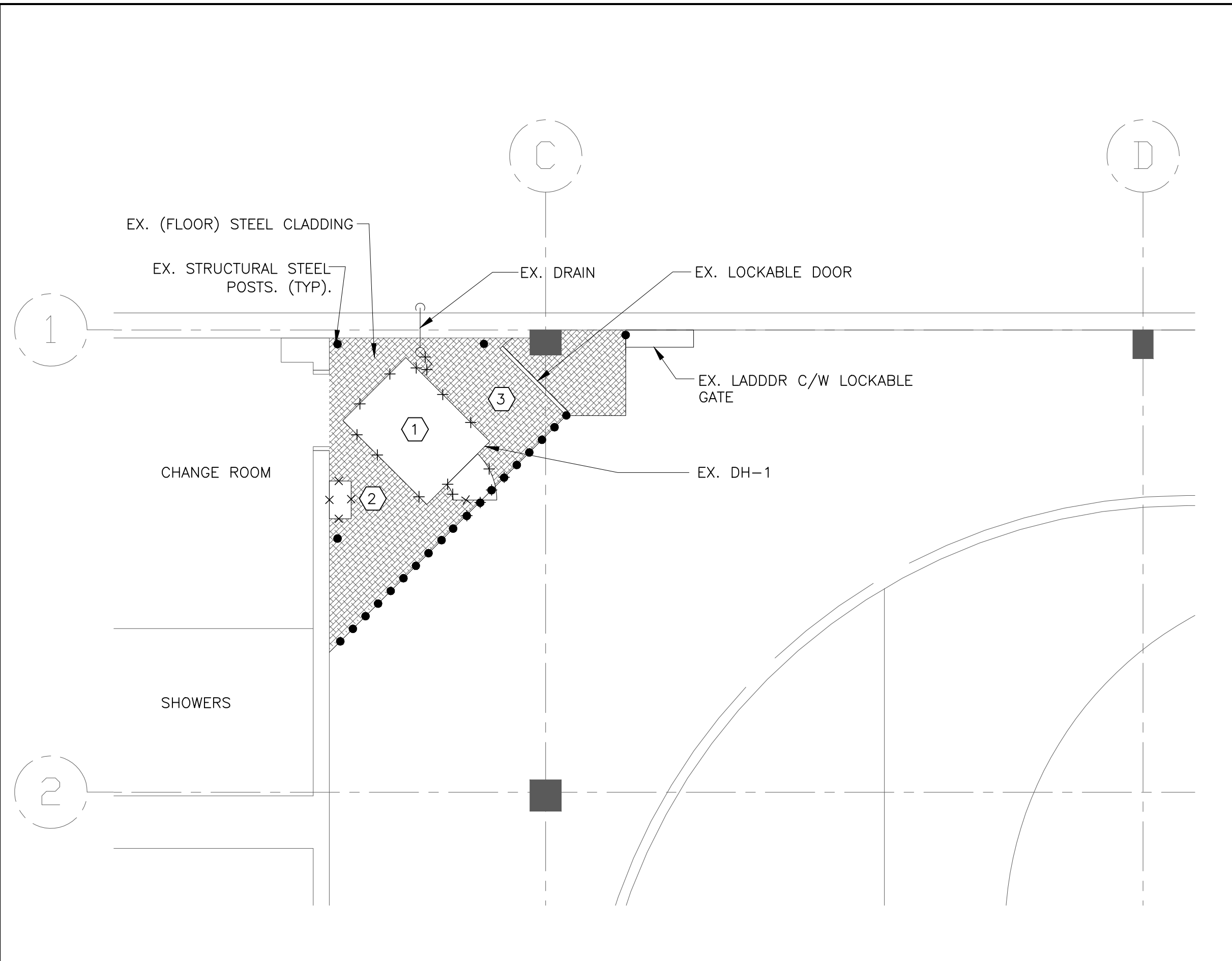
1 PART FLOOR PLAN HVAC – DEMOLITION M-6 SCALE: 1:50
