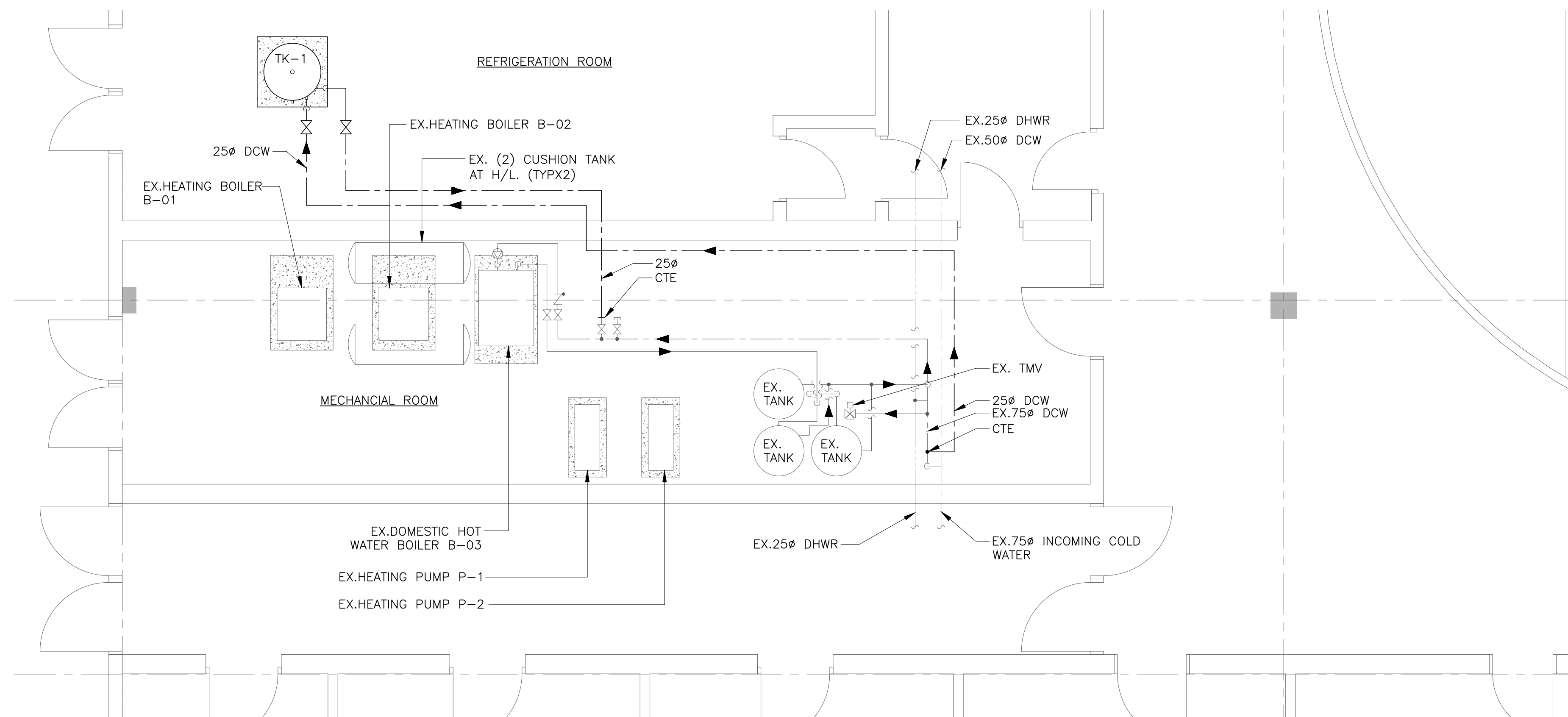
1 MECHANICAL ROOM PLUMBING – PROPOSED M-5 SCALE: 1:50
