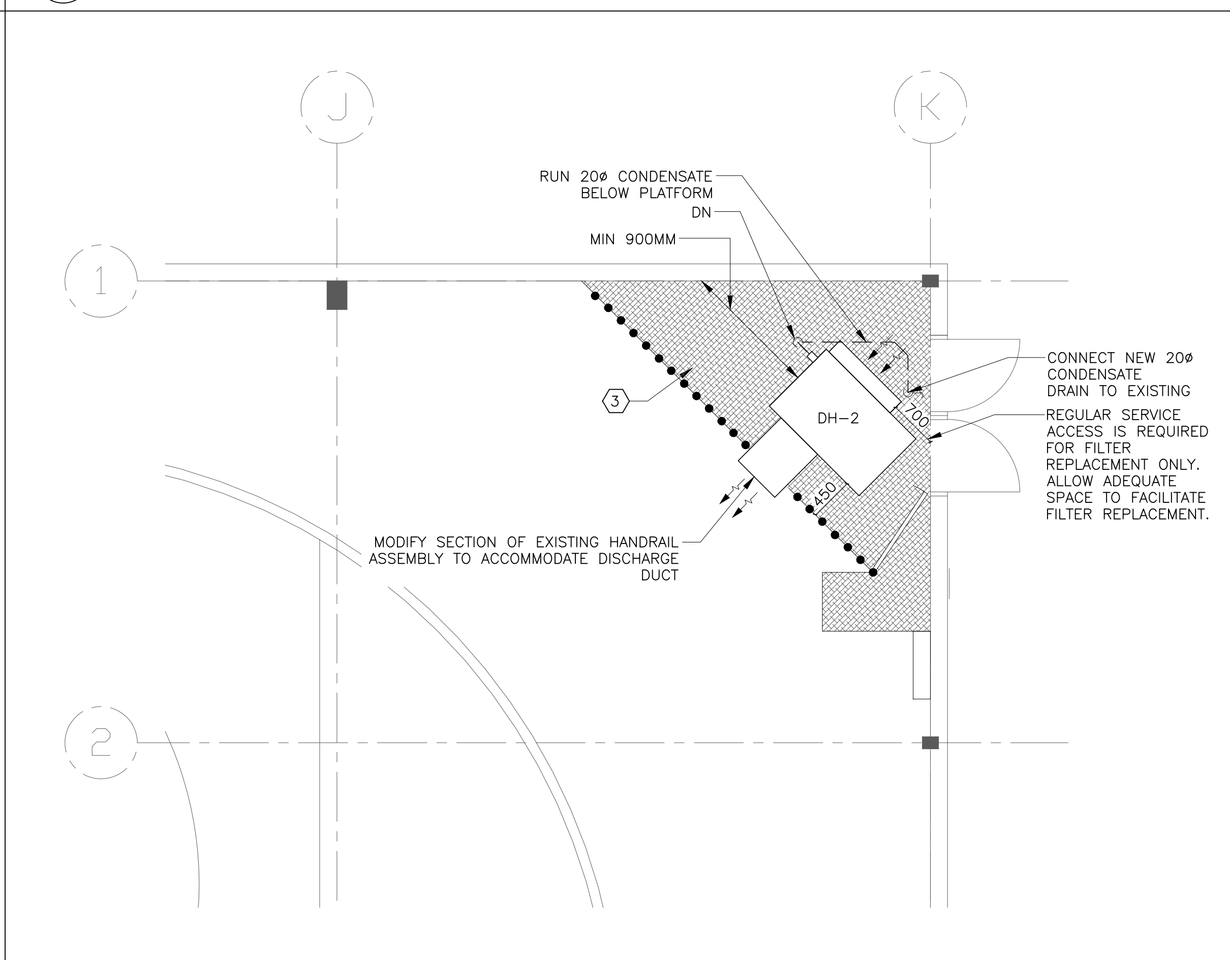
4 PART FLOOR PLAN HVAC – PROPOSED M-6 SCALE: 1:50
