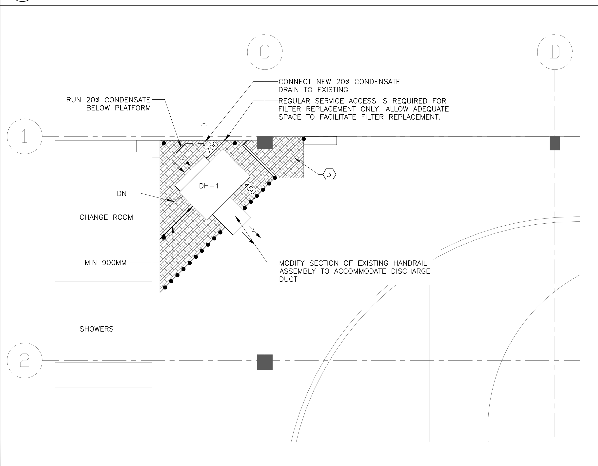
2 PART FLOOR PLAN HVAC – PROPOSED M-6 SCALE: 1:50
