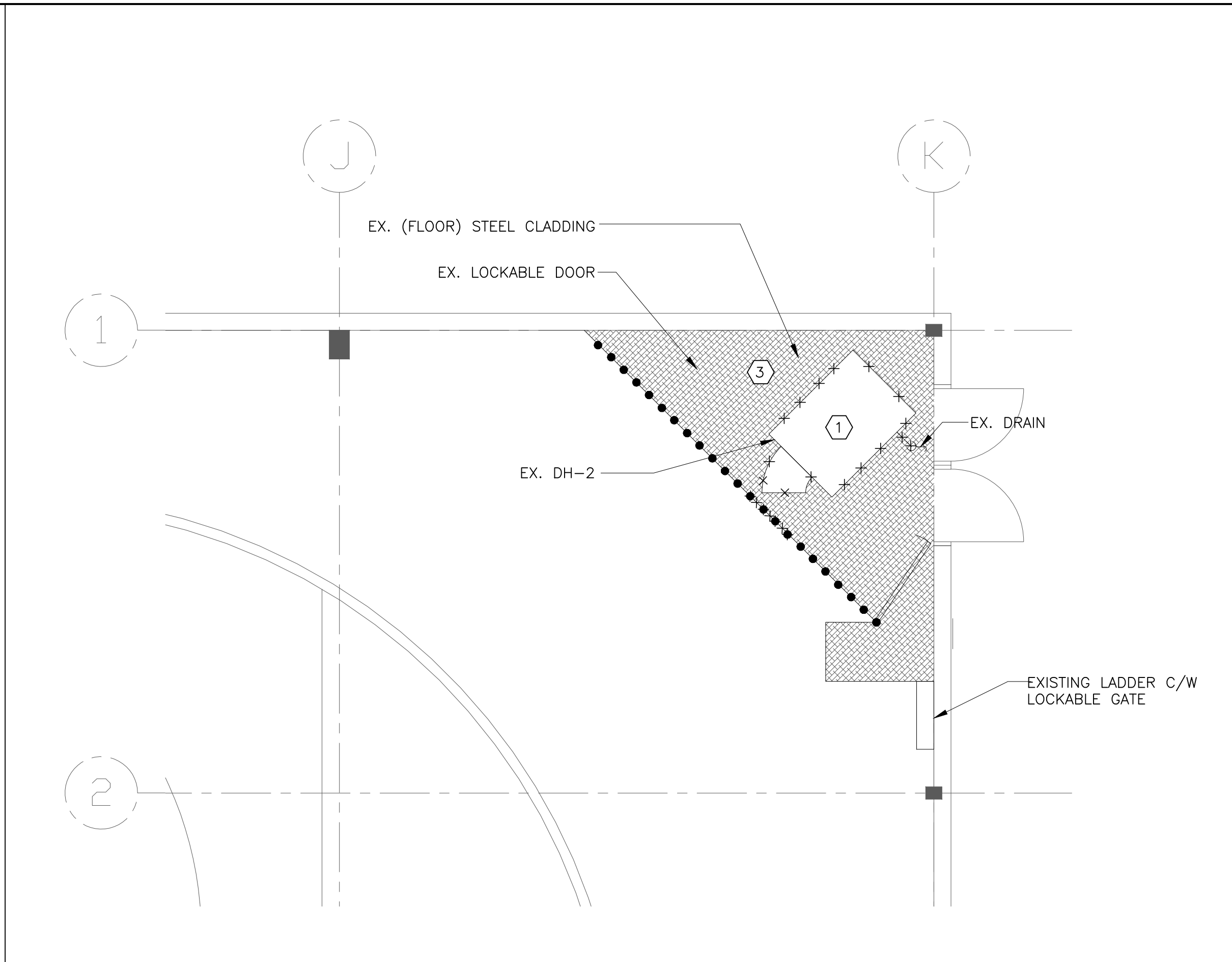
3 PART FLOOR PLAN HVAC – DEMOLITION M-6 SCALE: 1:50
