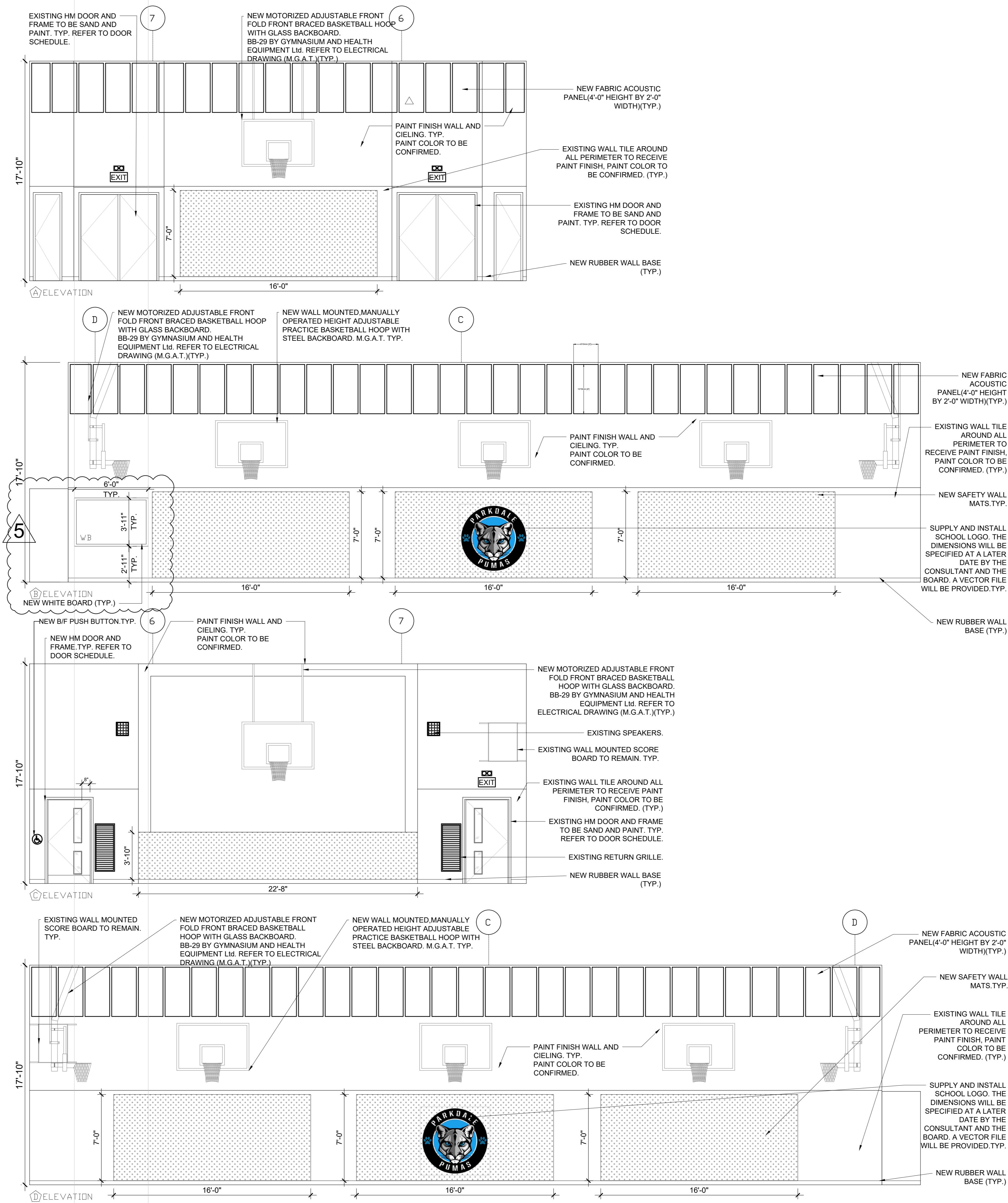
2 GYMNASIUM - INTERIOR ELEVATIONS SCALE: 1/4"=1'-0"
