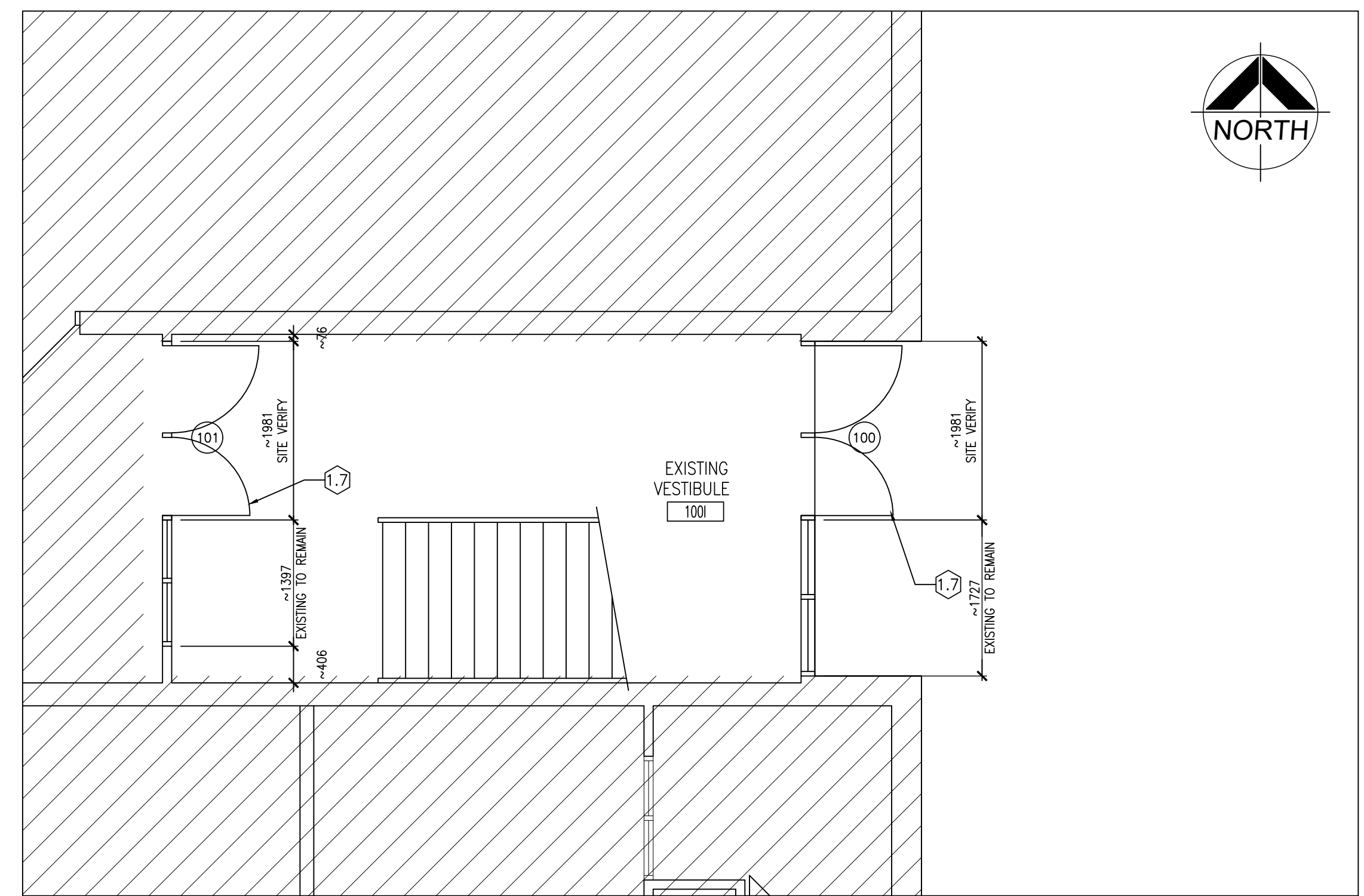
2 A207 PART FIRST FLOOR PLAN (DOOR 100) 1:50
