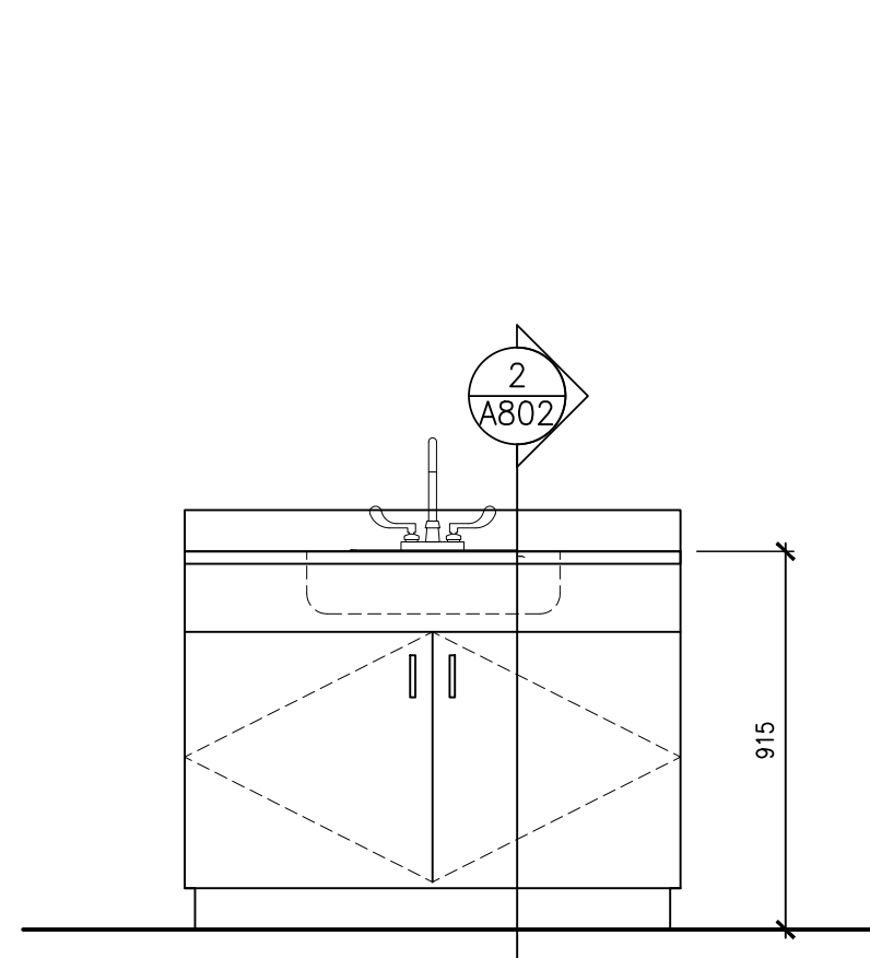
ML-2 ELEVATION
