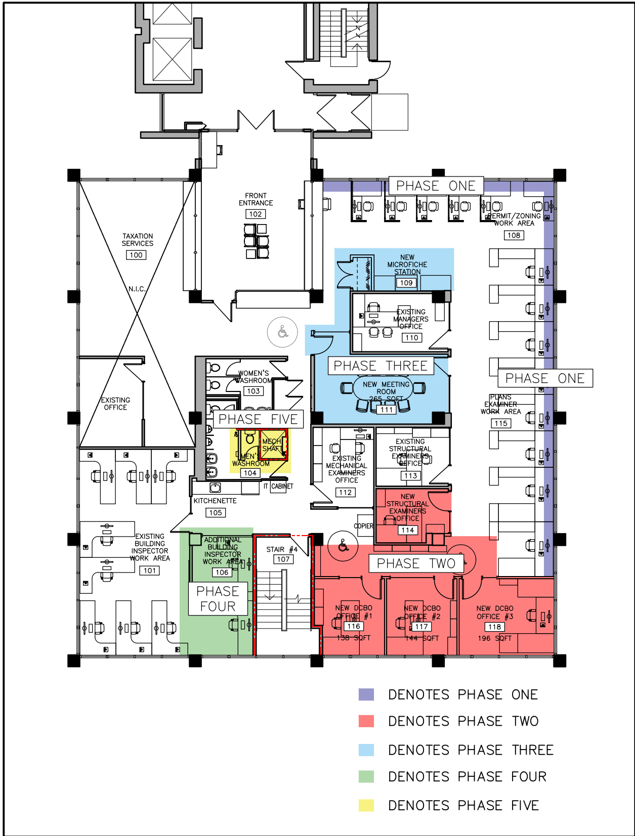
1 PHASING DIAGRAM ASK-01 SCALE: 1/16" = 1'-0"
