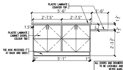
6 ISLAND ELEVATION
