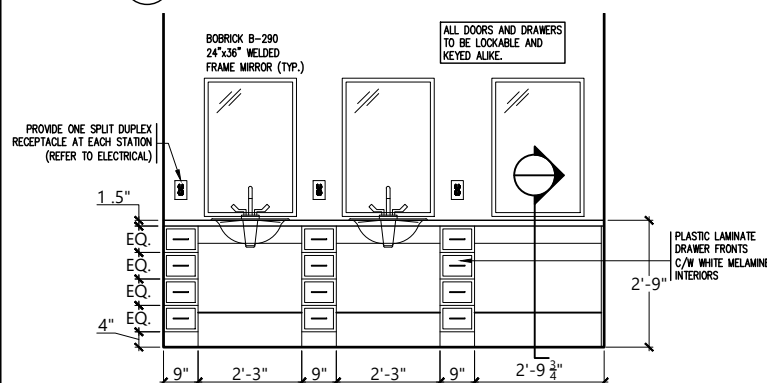
3 MILLWORK ELEVATION - BEAUTY AREA
