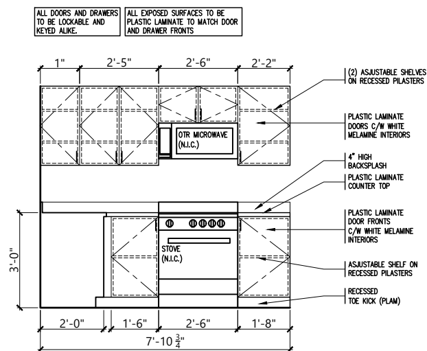
2 MILLWORK ELEVATION - KITCHEN
