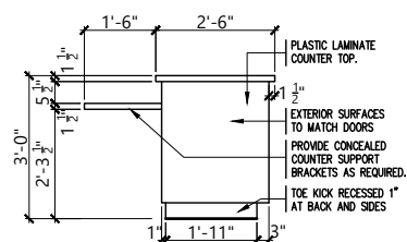
7 ISLAND ELEVATION
