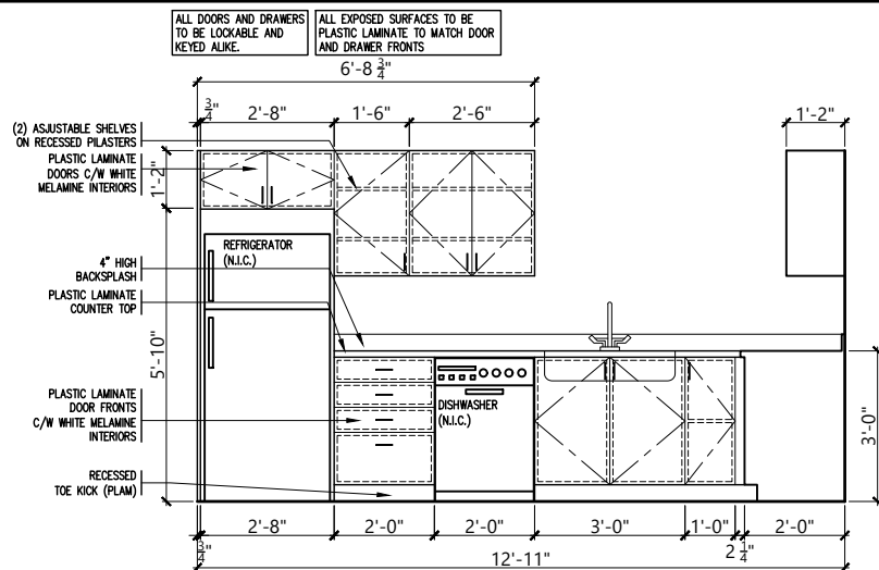
1 MILLWORK ELEVATION - KITCHEN
