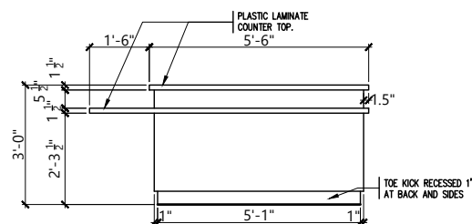
8 ISLAND ELEVATION
