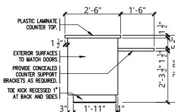
5 ISLAND ELEVATION
