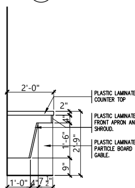
4 MILLWORK SECTION
