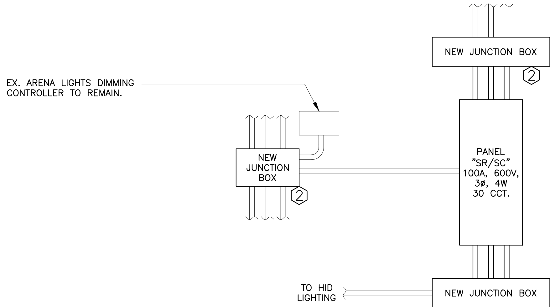
PROPOSED PLAN
