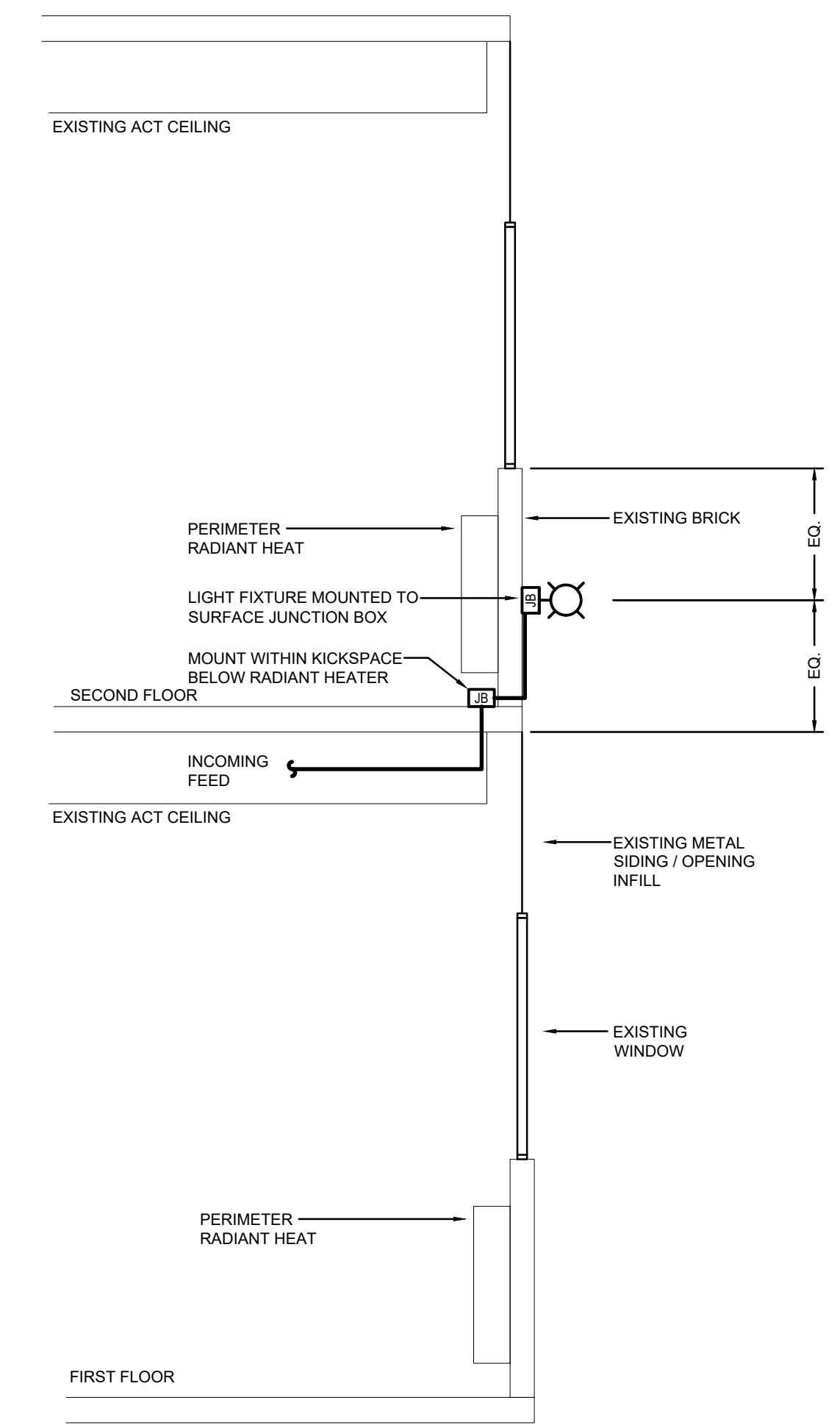
A-FIXTURE MOUNTING SECTION SCALE: 1:100
